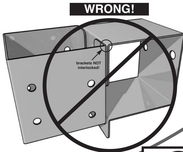
Example of a Cup-Loc bracket connection.
