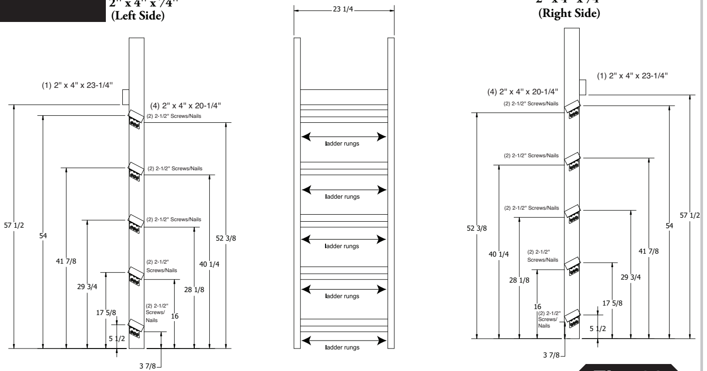
EXAMPLE OF LADDER RUNG INSTALLATION
