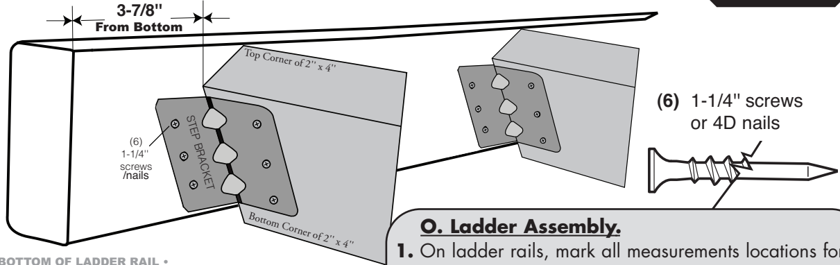
EXAMPLE OF LADDER RUNG INSTALLATION
