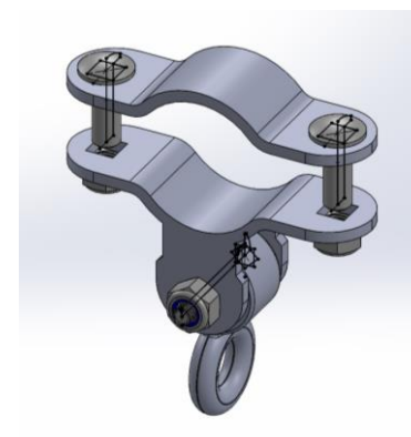
3 1/2" SWING HANGER
