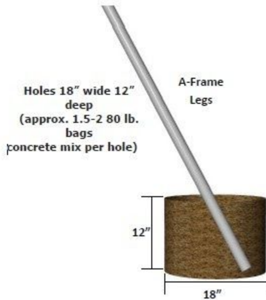
Hole Sizes for Cementing in the Set
